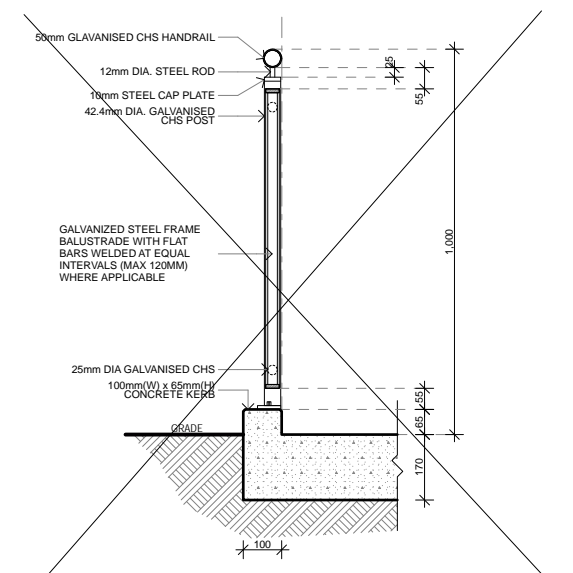
0 TYPICAL RAMP HANDRAIL DETAIL - SECTION 1:10
