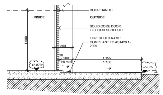
4 THRESHOLD RAMP DETAIL 1:20
