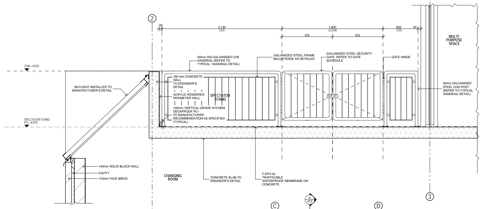
1 BALUSTRADE DETAIL 1:20
