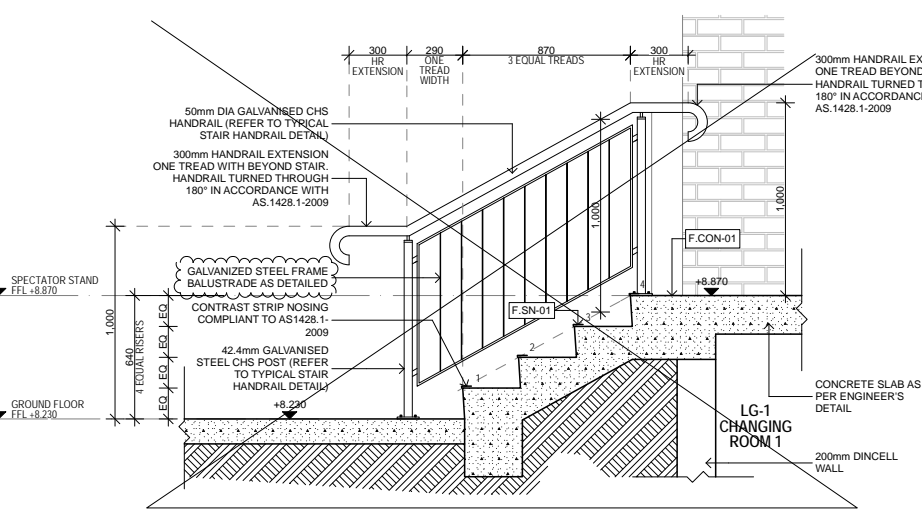
2 STAIR 1 - SECTION 1:20
