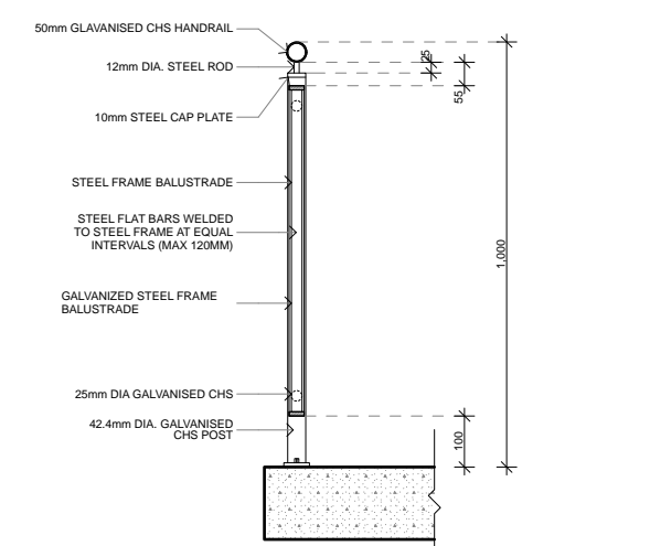
0 TYPICAL STAIR/BALUSTRADE DETAIL - SECTION 1:10
