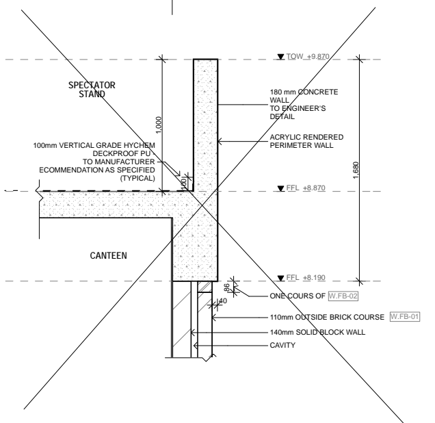
A SECTION DETAIL 1:20
