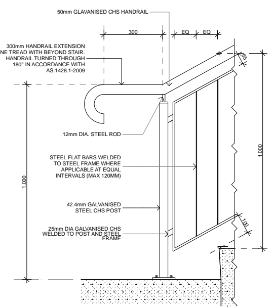
0 TYPICAL RAMP HANDRAIL DETAIL - ELEVATION 1:10
